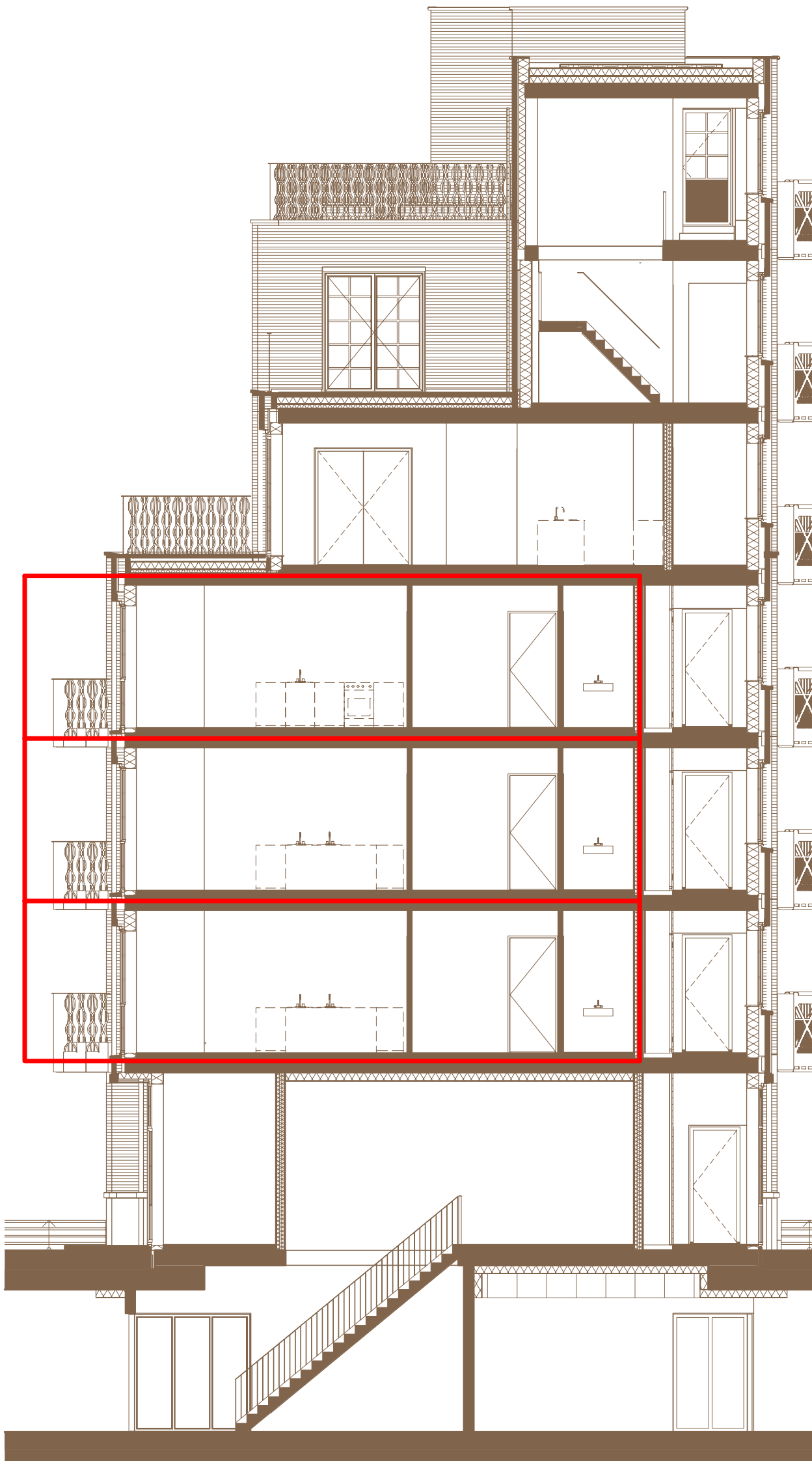
Doorsnede The Estate
