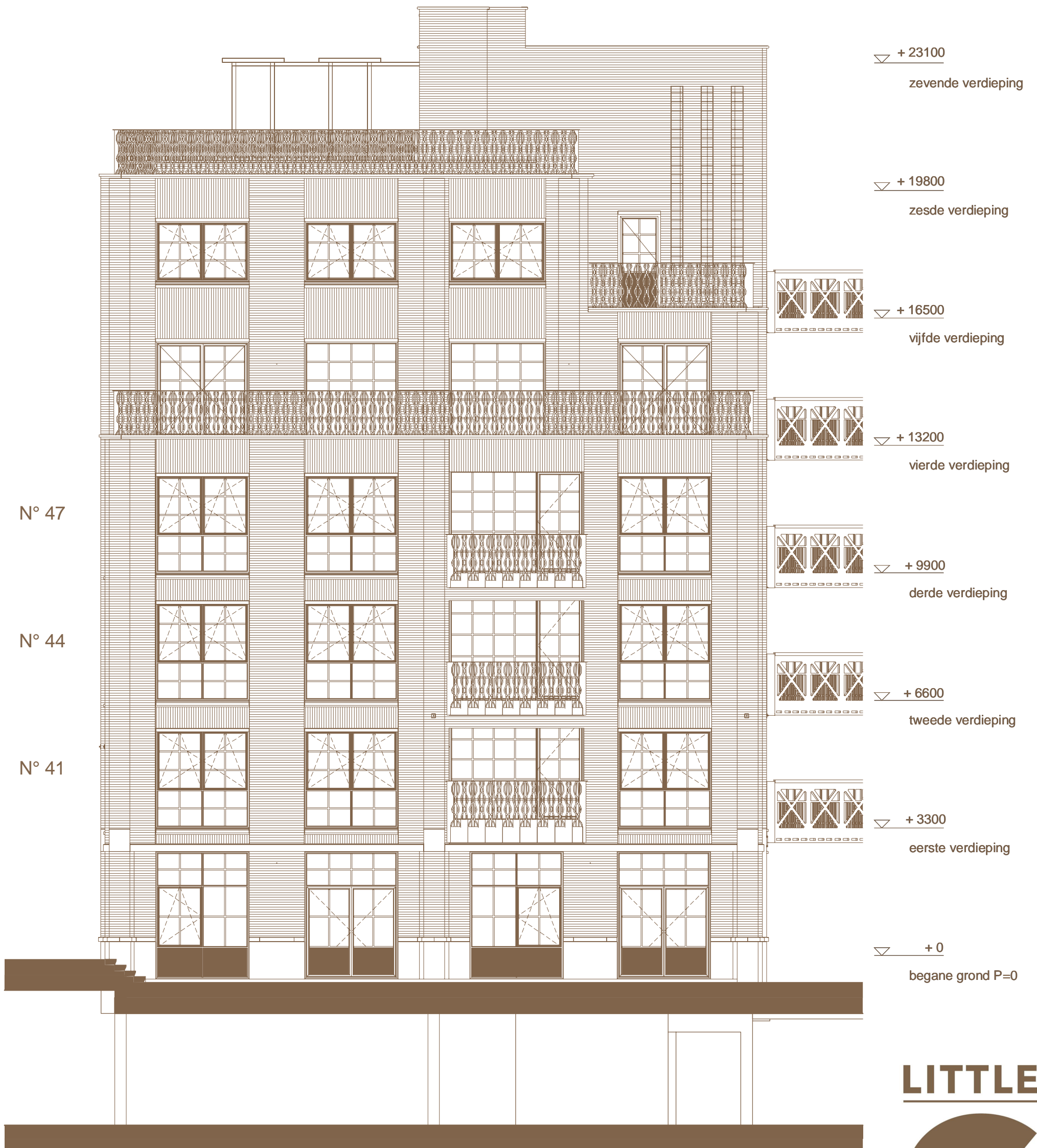
Noordgevel The Estate
