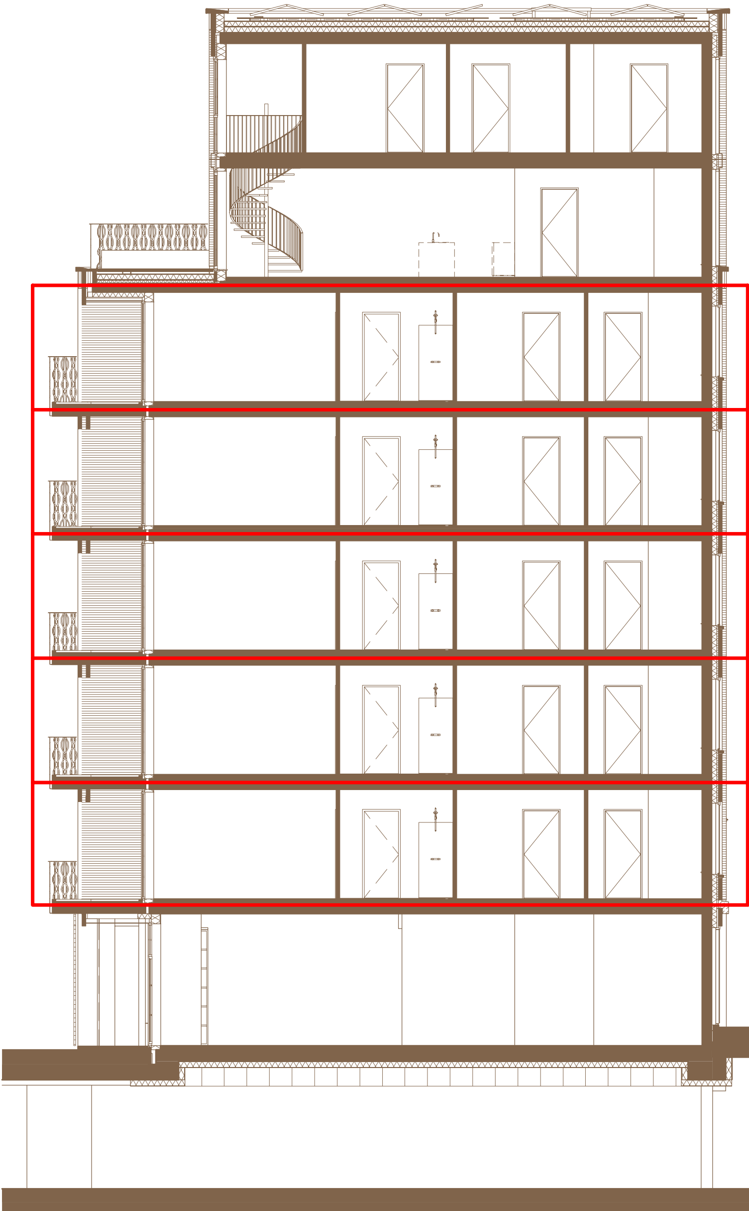
Doorsnede The Central
