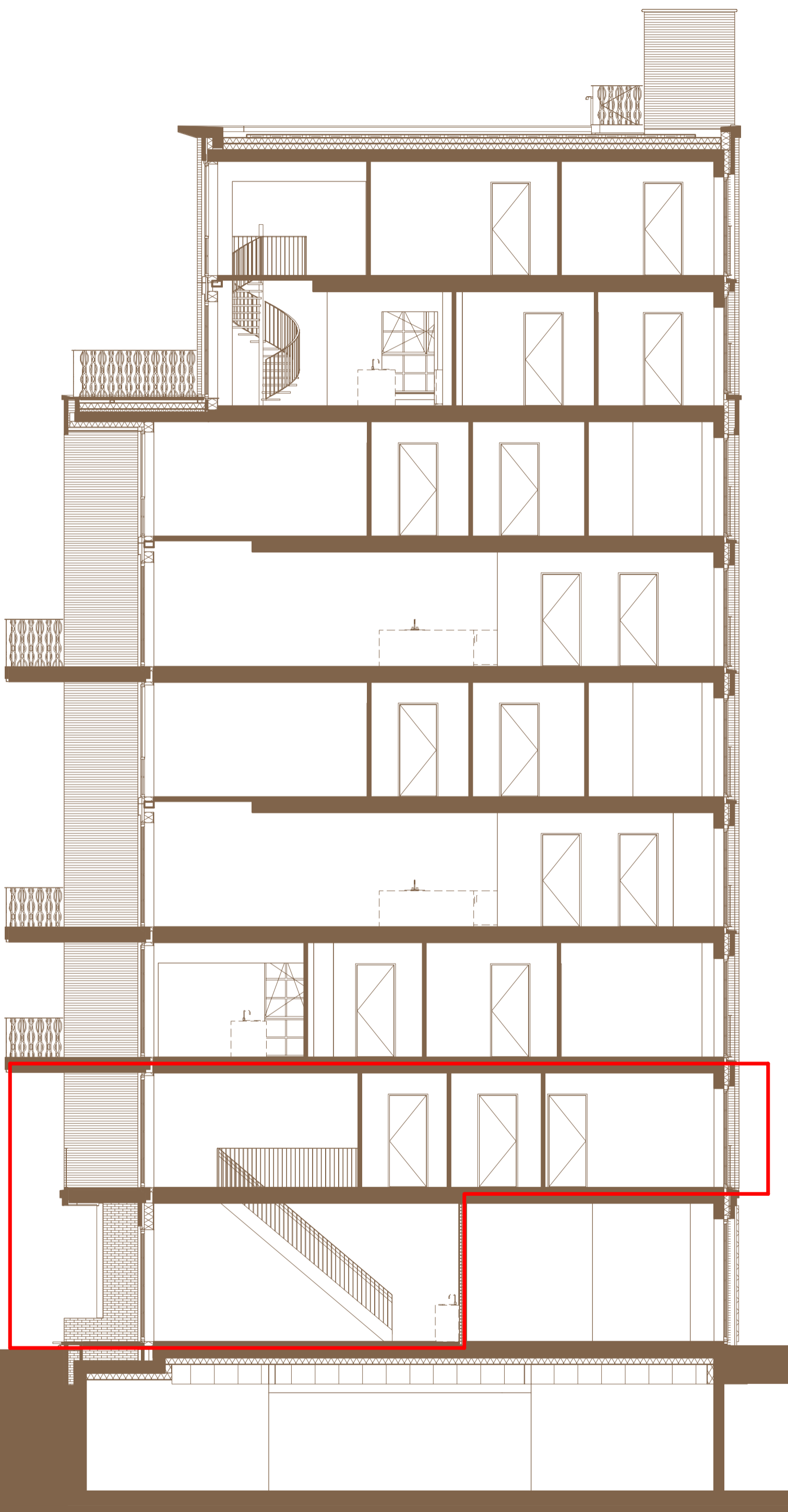
Doorsnede The Metropolitan
