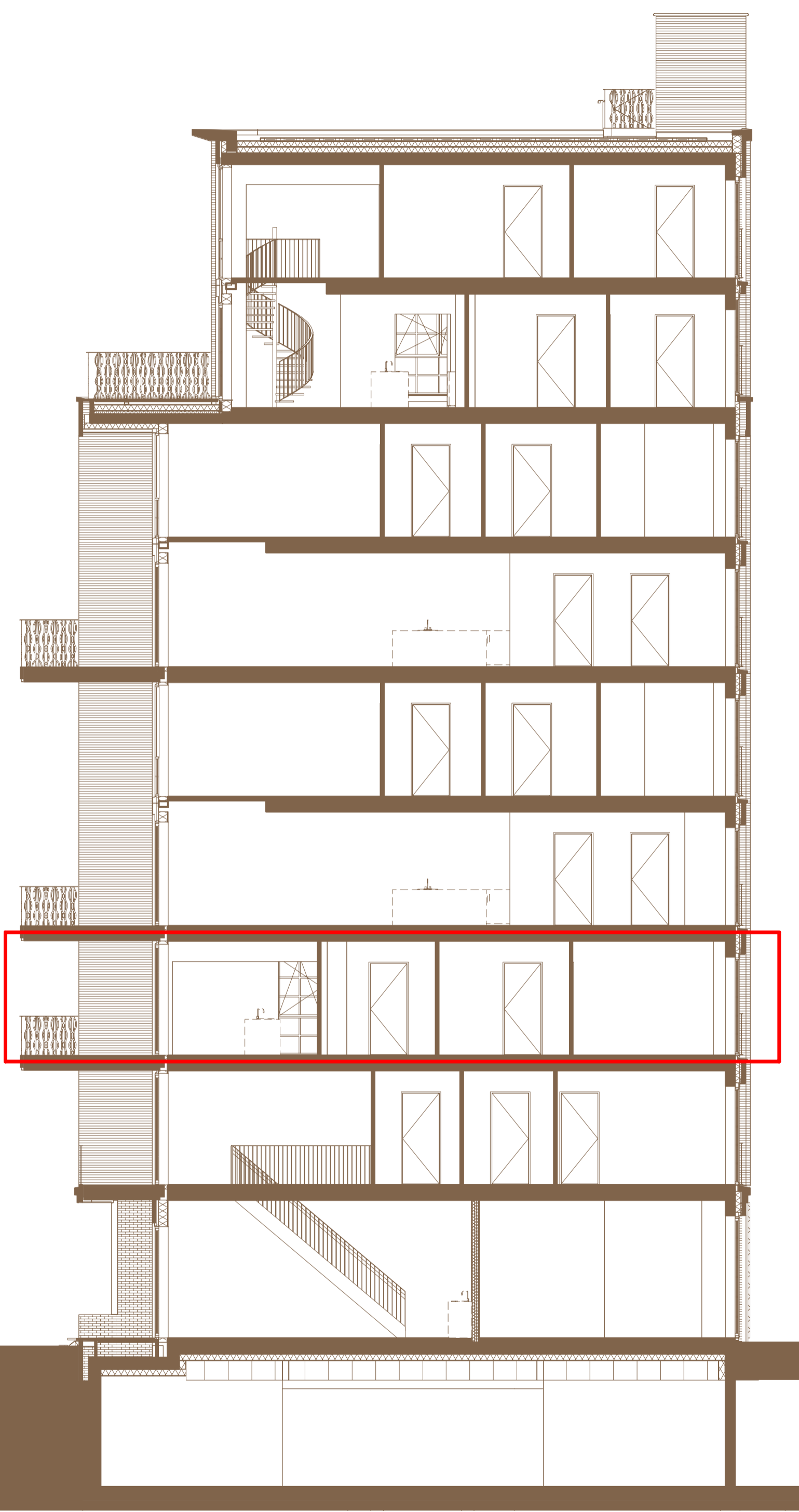
Doorsnede The Metropolitan
